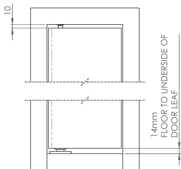
ELEVATION - DOOR LEAF CLOSED
